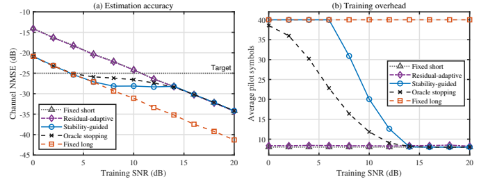
Fig. 5. Stability-guided adaptive training with the practical Algorithm 1 initialization: (a) channel NMSE and (b) average selected pilot symbols versus training SNR. The fixed-short and fixed-long schemes use T_p = 8 and 40, respectively; oracle stopping uses the true channel error only as an unattainable benchmark. Each point averages 300 paired trials.
