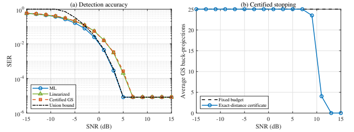
Fig. 6. Perfect-CSI detection: (a) SER of ML, linearized, and GS detectors together with the analytical distance-spectrum union bound, and (b) average GS back-projections with a fixed budget and the exact d_{\min}^{(E)} certificate.
