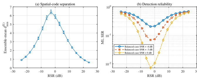
Fig. 11. Effect of the reference-to-signal energy ratio under a fixed total incident-energy budget: (a) ensemble-mean minimum energy distance over balanced spatial phase maps and (b) perfect-CSI ML SER at three balanced-case SNRs. Error bars show one standard deviation across phase maps.
