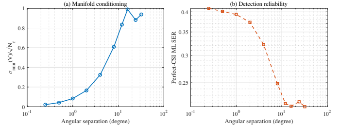
Fig. 10. Effect of user angular separation on (a) array-manifold conditioning and (b) perfect-CSI ML detection at -6 dB.
