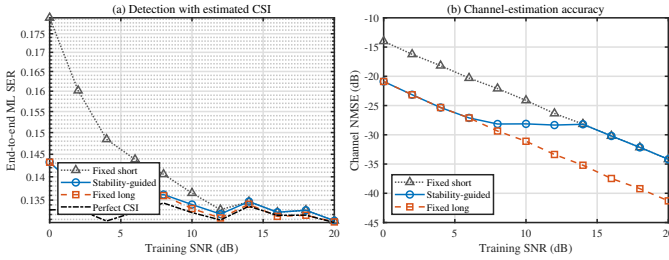
Fig. 8. End-to-end comparison versus training SNR: (a) SER of the fixed-short, stability-guided, and fixed-long training policies with perfect-CSI ML as a benchmark and (b) their channel NMSE. The data SNR is 0 dB.
