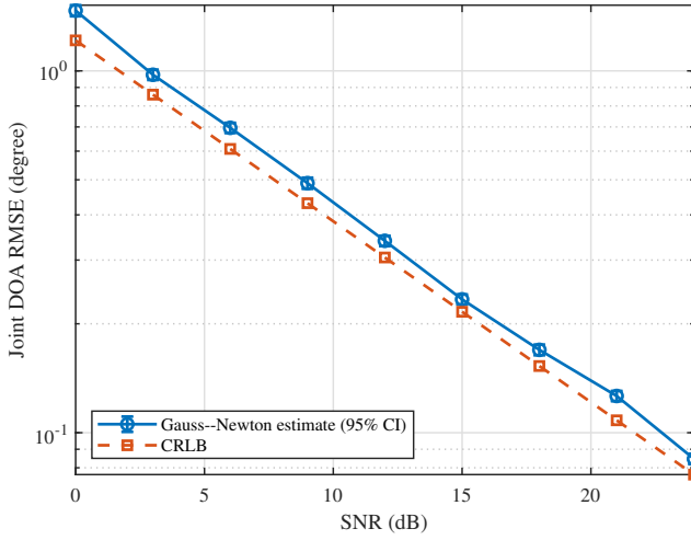
Fig. 3. Joint DOA RMSE and the corresponding CRLB versus SNR under the fixed spatial four-phase reference code. Error bars show 95% confidence intervals.
