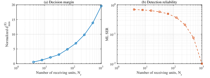
Fig. 9. Effect of the number of receiving units on (a) the normalized energy-domain minimum distance and (b) perfect-CSI ML detection at -12 dB.
