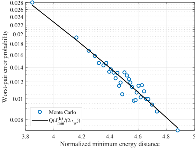
Fig. 7. Worst-pair error probability versus normalized energy-domain minimum distance over equal-power fixed spatial phase maps.
