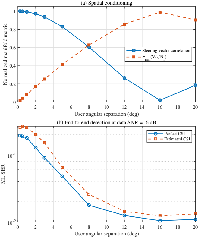
Fig. 16: Effect of user angular separation on (a) array-manifold conditioning and (b) end-to-end ML detection.
