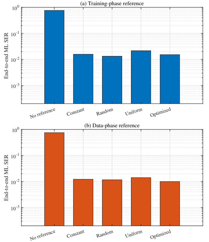
Fig. 13: End-to-end ML SER for different (a) training-phase and (b) data-phase reference designs.
