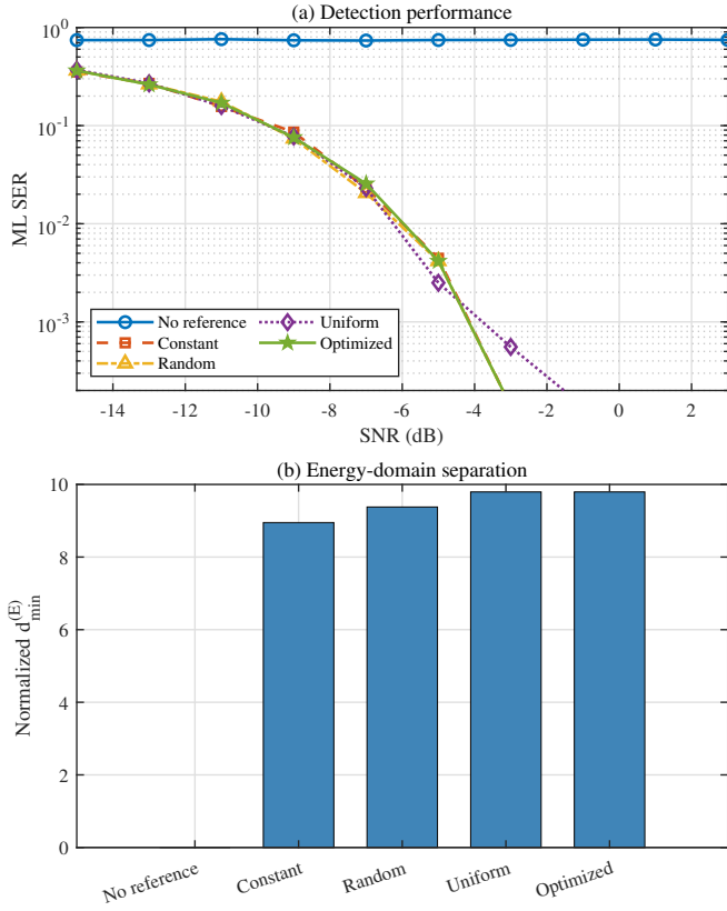
Fig. 8: Effect of the data-phase reference: (a) ML SER and (b) normalized energy-domain minimum distance.
