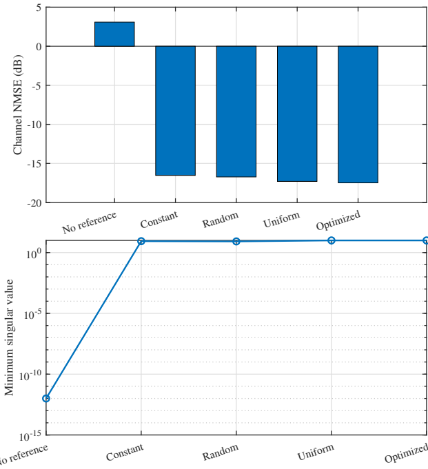
Fig. 6: Channel NMSE and minimum Jacobian singular value for different reference designs.
