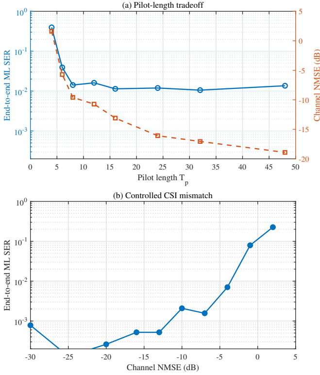
Fig. 12: Effect of channel-estimation accuracy on end-to-end ML detection: (a) pilot-length tradeoff and (b) controlled CSI mismatch.
