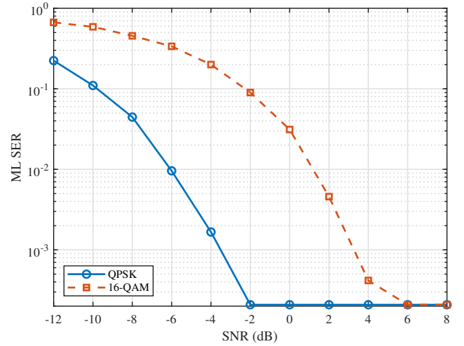
Fig. 10: ML SER for QPSK and 16-QAM under perfect CSI.
