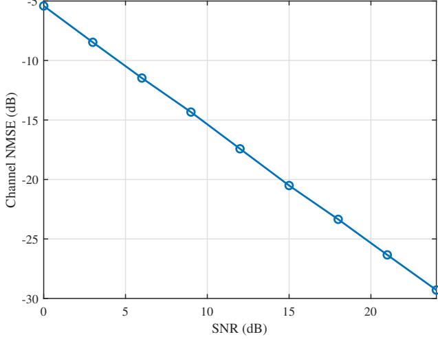
Fig. 2: Channel-estimation NMSE versus intensity-domain SNR.
