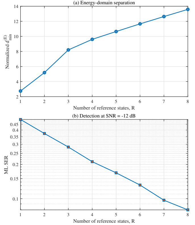
Fig. 15: Effect of the number of phase-shifted reference states on (a) the normalized energy-domain minimum distance and (b) ML detection.
