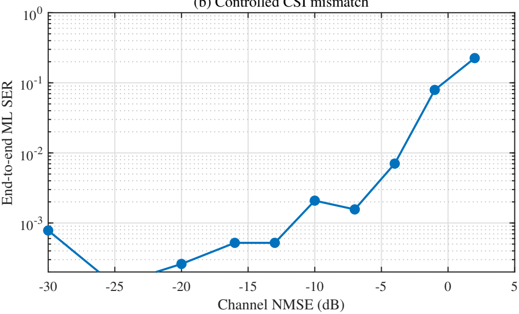
(b) Controlled CSI mismatch
