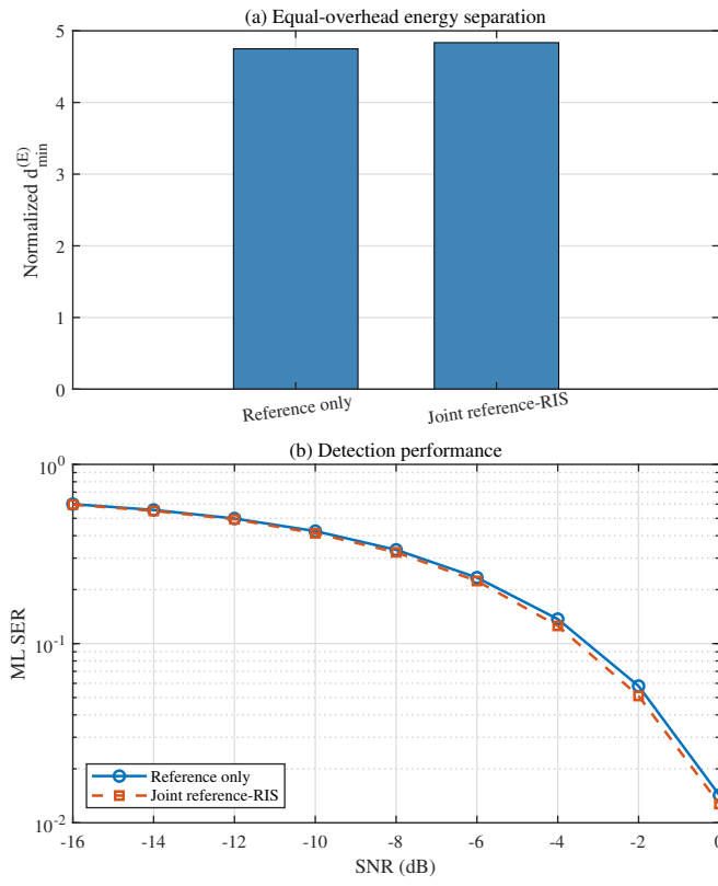
Fig. 17: Equal-overhead comparison of reference-only and joint reference-RIS measurement diversity: (a) normalized minimum distance and (b) ML SER.
