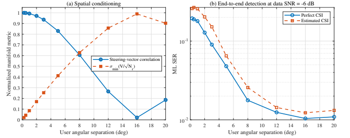
Fig. 14: Effect of user angular separation on (a) array-manifold conditioning and (b) end-to-end ML detection.
