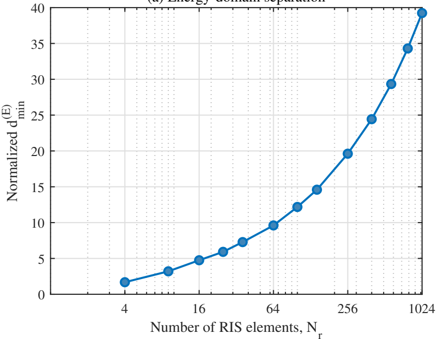
(a) Energy-domain separation
