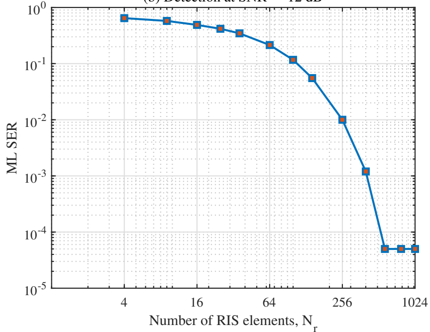
(b) Detection at SNR = -12 dB
