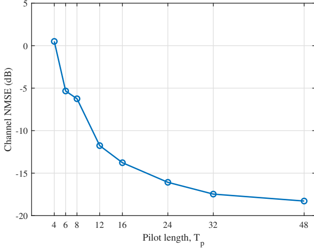
Fig. 4: Channel-estimation NMSE versus pilot length at an SNR of 12 dB.
