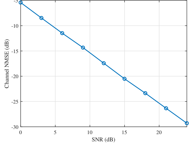
Fig. 2: Channel-estimation NMSE versus intensity-domain SNR.
