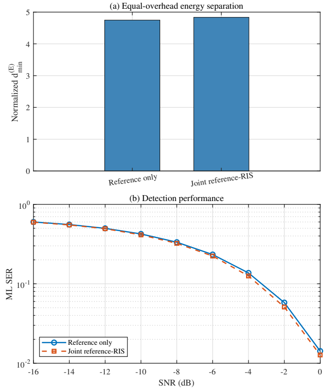
Fig. 17: Equal-overhead comparison of reference-only and joint reference-RIS measurement diversity: (a) normalized minimum distance and (b) ML SER.
