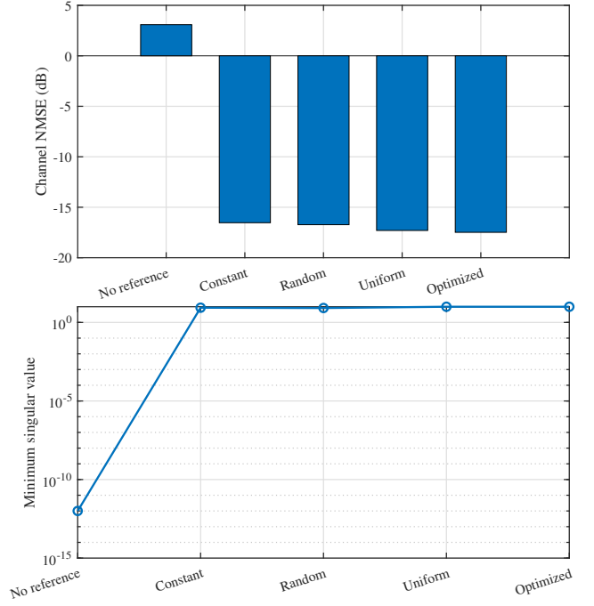
Fig. 6: Channel NMSE and minimum Jacobian singular value for different reference designs.
