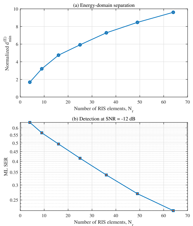
Fig. 14: Effect of the number of RIS element-level observations on (a) the normalized energy-domain minimum distance and (b) ML detection.
