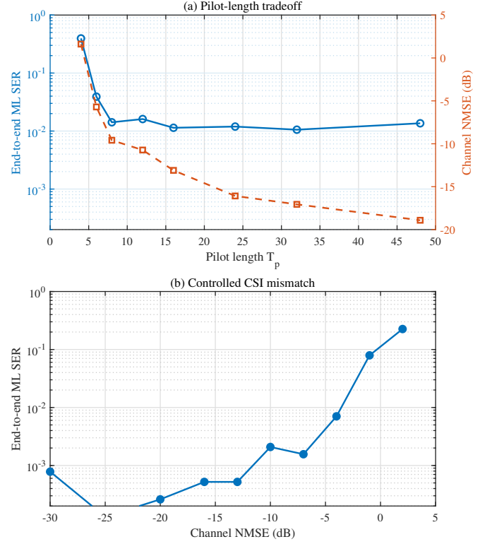
Fig. 12: Effect of channel-estimation accuracy on end-to-end ML detection: (a) pilot-length tradeoff and (b) controlled CSI mismatch.
