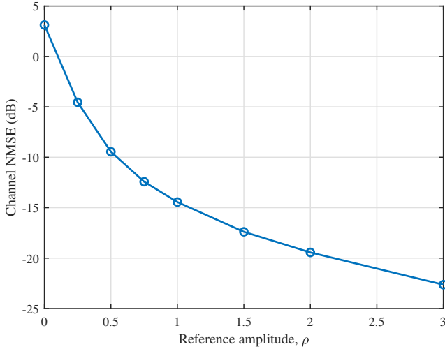
Fig. 5: Channel-estimation NMSE versus reference amplitude for fixed post-detection noise variance.
