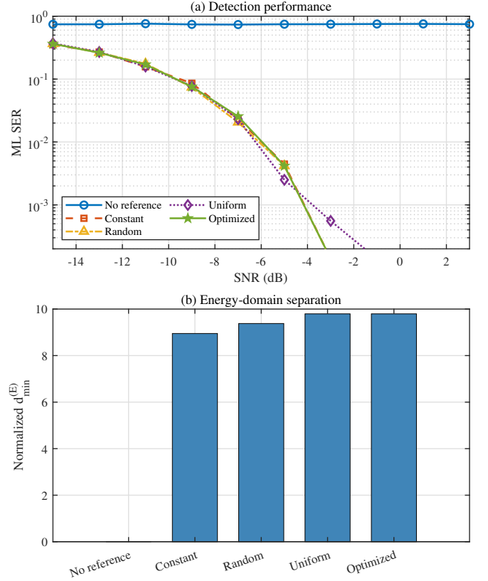
Fig. 8: Effect of the data-phase reference: (a) ML SER and (b) normalized energy-domain minimum distance.
