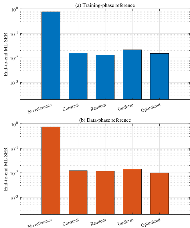
Fig. 13: End-to-end ML SER for different (a) training-phase and (b) data-phase reference designs.
