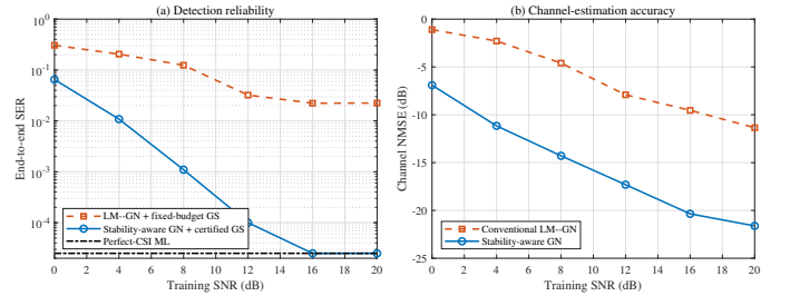
Fig. 8. End-to-end comparison versus training SNR: (a) SER of the conventional and theory-guided receivers with perfect-CSI ML as a benchmark and (b) channel NMSE of conventional LM-GN and stability-aware GN. The data SNR is 12 dB; zero-error SERs are shown at the half-event level.
