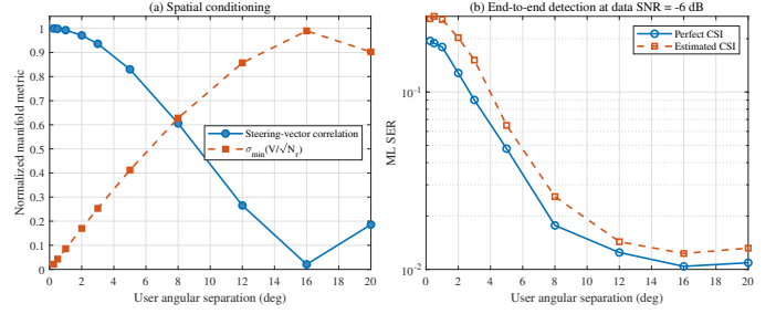
Fig. 15. Effect of user angular separation on (a) array-manifold conditioning and (b) end-to-end ML detection.
