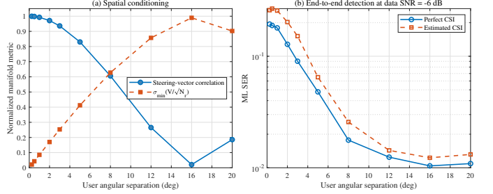
Fig. 11. Effect of user angular separation on (a) array-manifold conditioning and (b) end-to-end ML detection.
