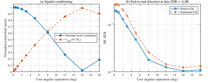
Fig. 15. Effect of user angular separation on (a) array-manifold conditioning and (b) end-to-end ML detection.
