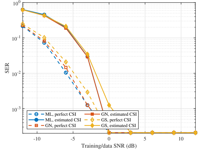
Fig. 11. SER under perfect and estimated CSI for different symbol detectors.
