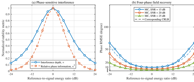
Fig. 17. Effect of the reference-to-signal energy ratio under a fixed total incident-energy budget: (a) normalized interference depth and relative phase information and (b) phase RMSE of four-phase field recovery. Solid curves with markers are Monte Carlo results, dashed curves are the corresponding CRLBs, and the horizontal dotted line denotes a 10^\circ RMSE criterion.
