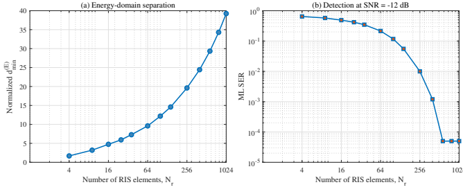
Fig. 13. Effect of the number of RIS element-level observations on (a) the normalized energy-domain minimum distance and (b) ML detection at -12 dB. Zero-error points are displayed at the half-event level.
