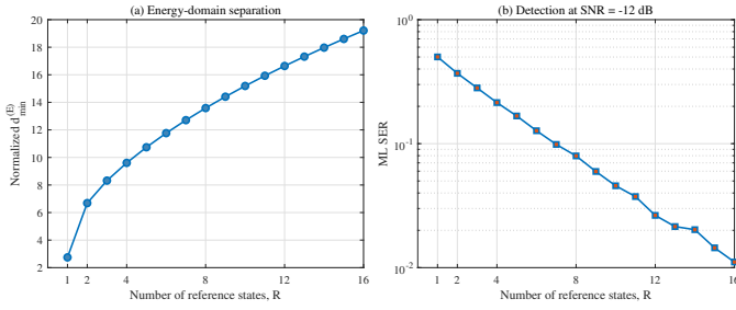
Fig. 13: Effect of the number of phase-shifted reference states on (a) the normalized energy-domain minimum distance and (b) ML detection.
