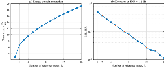
Fig. 10. Effect of the number of phase-shifted reference states on (a) the normalized energy-domain minimum distance and (b) ML detection.
