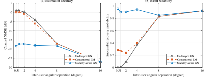
Fig. 5. Effect of inter-user angular separation on (a) channel NMSE and (b) successful recovery probability for undamped GN, conventional LM, and stability-aware GN. The stress test uses T_p = 16 , an SNR of 12 dB, and 300 paired trials; success denotes a joint DOA RMSE below 1^\circ .
