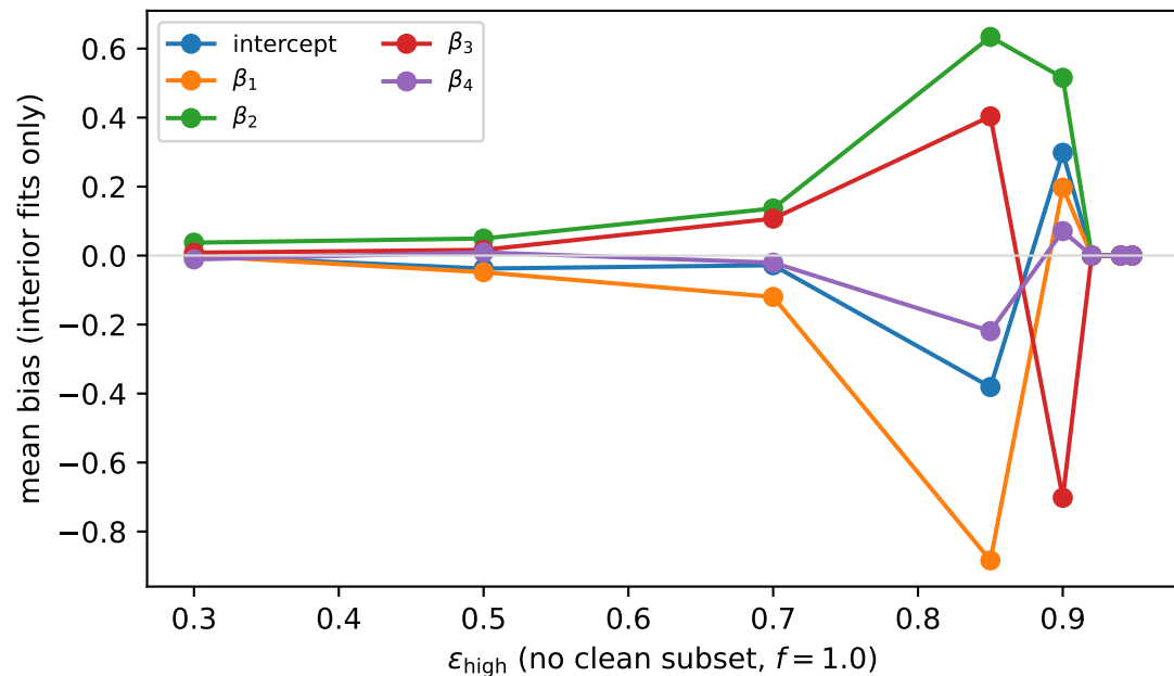
Per- i corrected bias on interior fits
