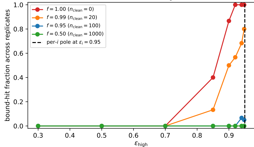
Identification limit as \varepsilon_{\text{high}} \rightarrow \text{pole}
