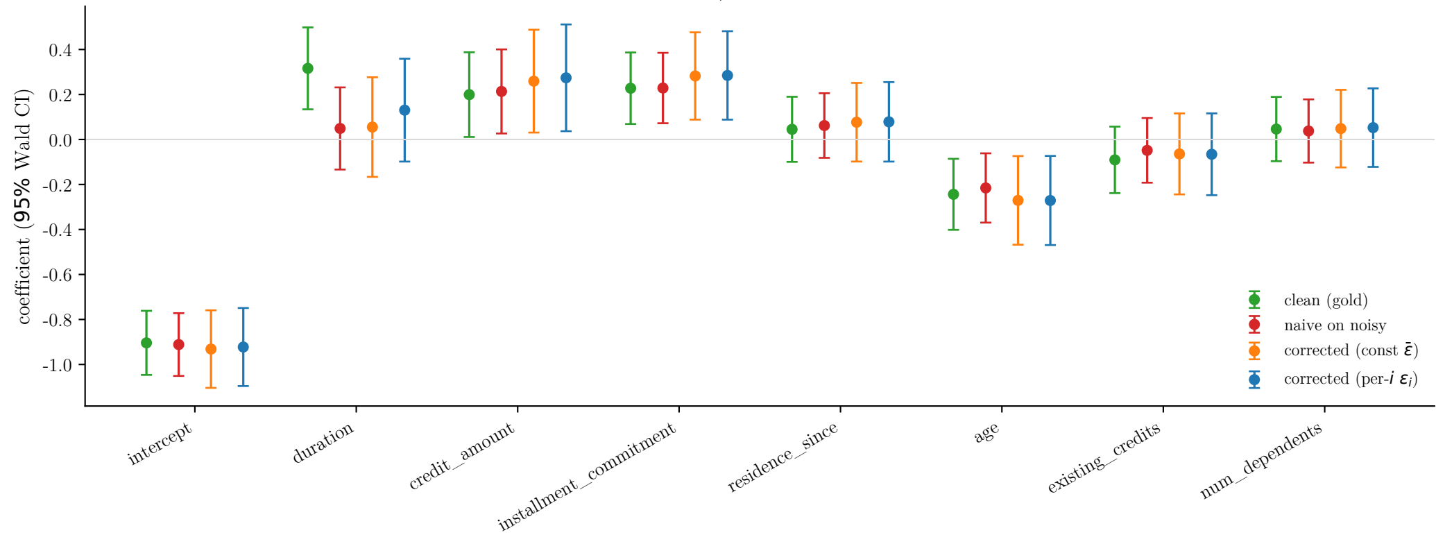
German Credit: corrected MLE vs. \ naive under duration-dependent label noise
