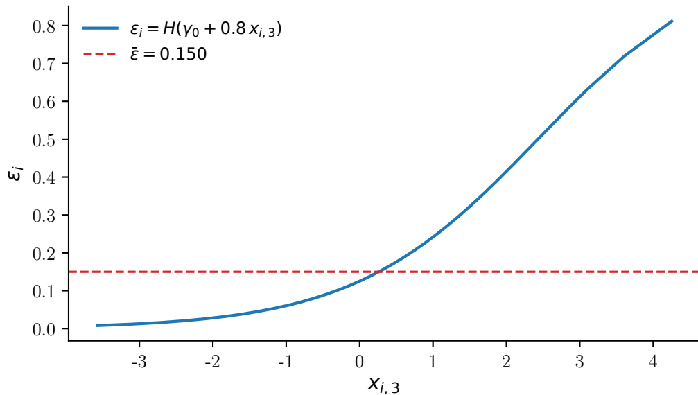
Per-observation flip rate vs. x_3
