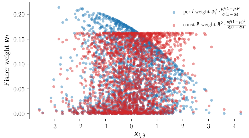
Per-observation Fisher weight at \beta^*
