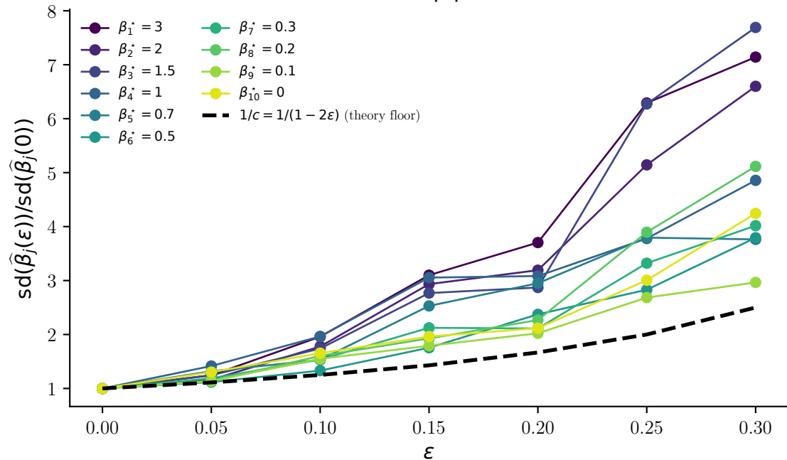
Relative inflation: 1/|c| is a lower bound
