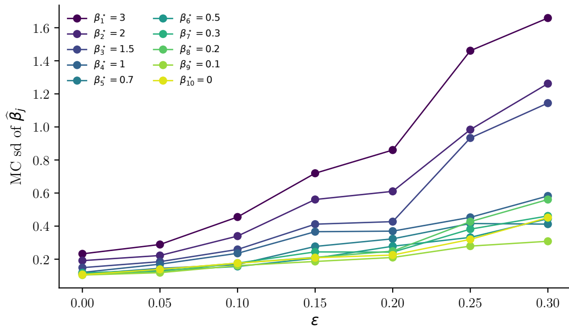
Absolute MC standard deviation
