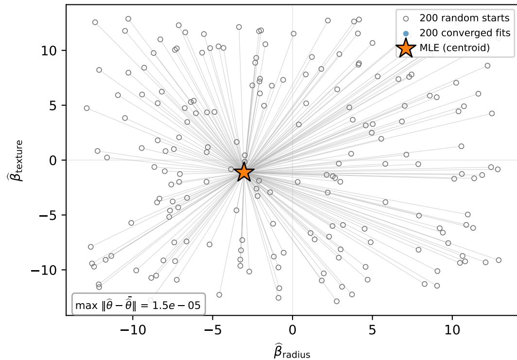
Breast cancer (4 predictors), \varepsilon = \delta = 0.10
