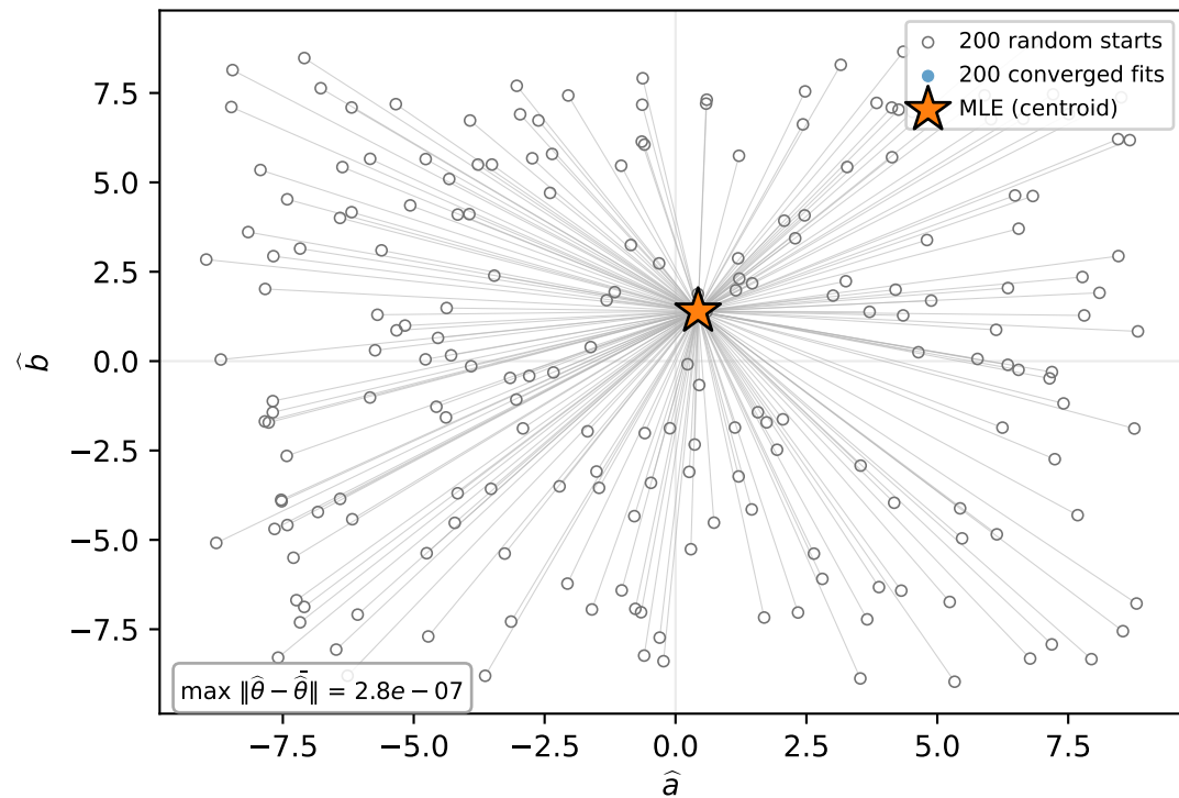
Synthetic single-covariate, \varepsilon = \delta = 0.10 , n = 1000
