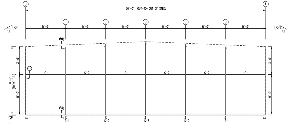
ENDWALL FRAMING FRAME LINE: 31
