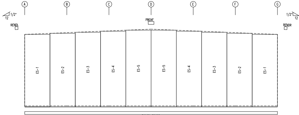
ENDWALL SHEETING & TRIM FRAME LINE: 1 PANELS: 26 Ga. RL - NEED COLOR
