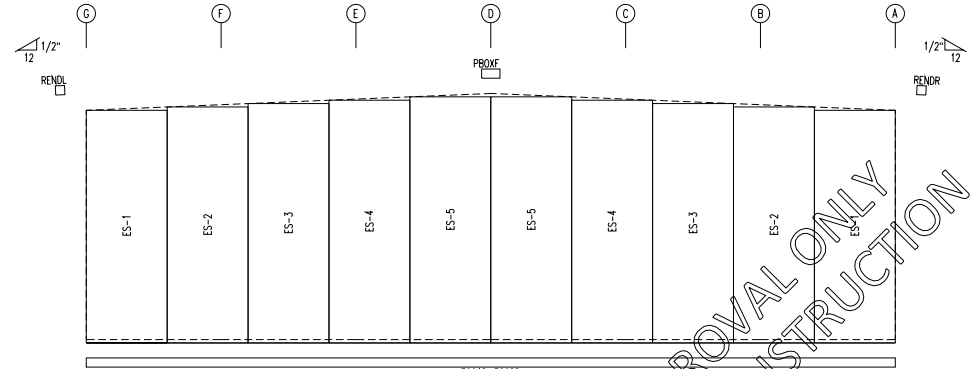
ENDWALL SHEETING & TRIM FRAME LINE: 31 PANELS: 26 Ga. RL - NEED COLOR
