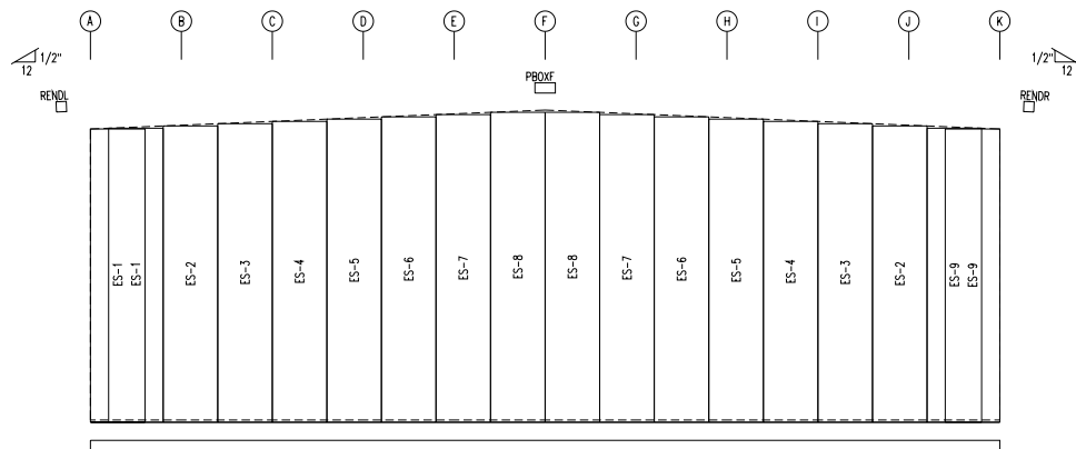
ENDWALL SHEETING & TRIM FRAME LINE: 1 PANELS: 26 Ga. RL - NEED COLOR
