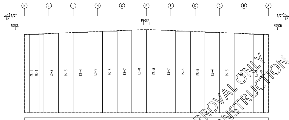
ENDWALL SHEETING & TRIM FRAME LINE: 31 PANELS: 26 Ga. RL - NEED COLOR
