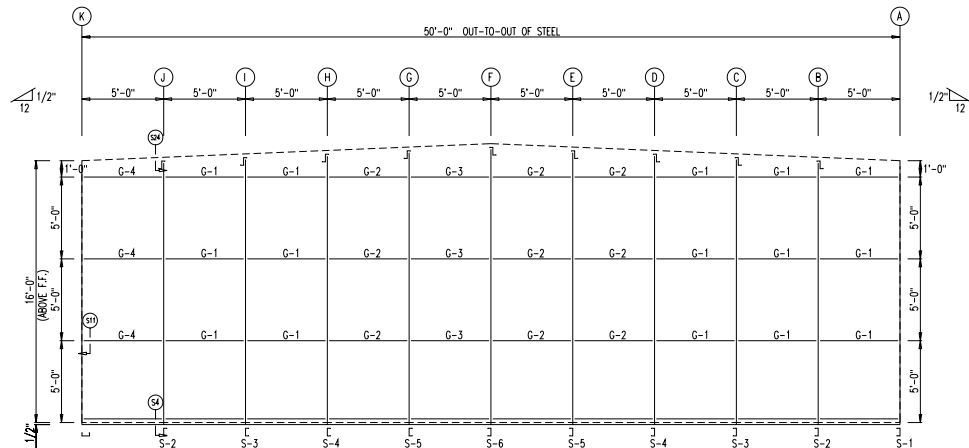
ENDWALL FRAMING FRAME LINE: 31
