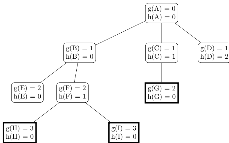
Figure 1: Sample search tree, labeled with costs g and heuristic values h . Boxes indicate goal nodes. A^* search returns the optimal goal node G.
