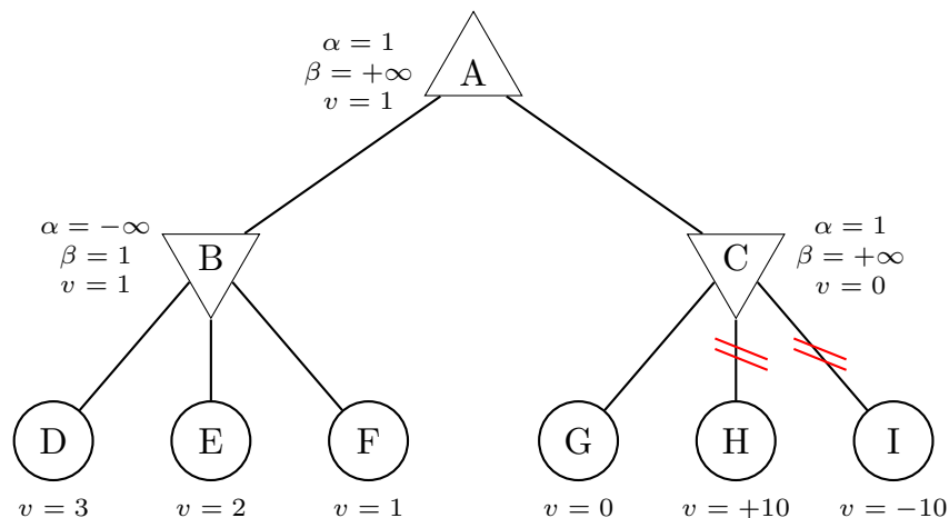
Figure 3: An example of \alpha\beta pruning. The subtrees rooted at H and I can be pruned because their values do not impact the value of node A . Indeed, the pruning test passes: v = 0 \leq 1 = \alpha .
