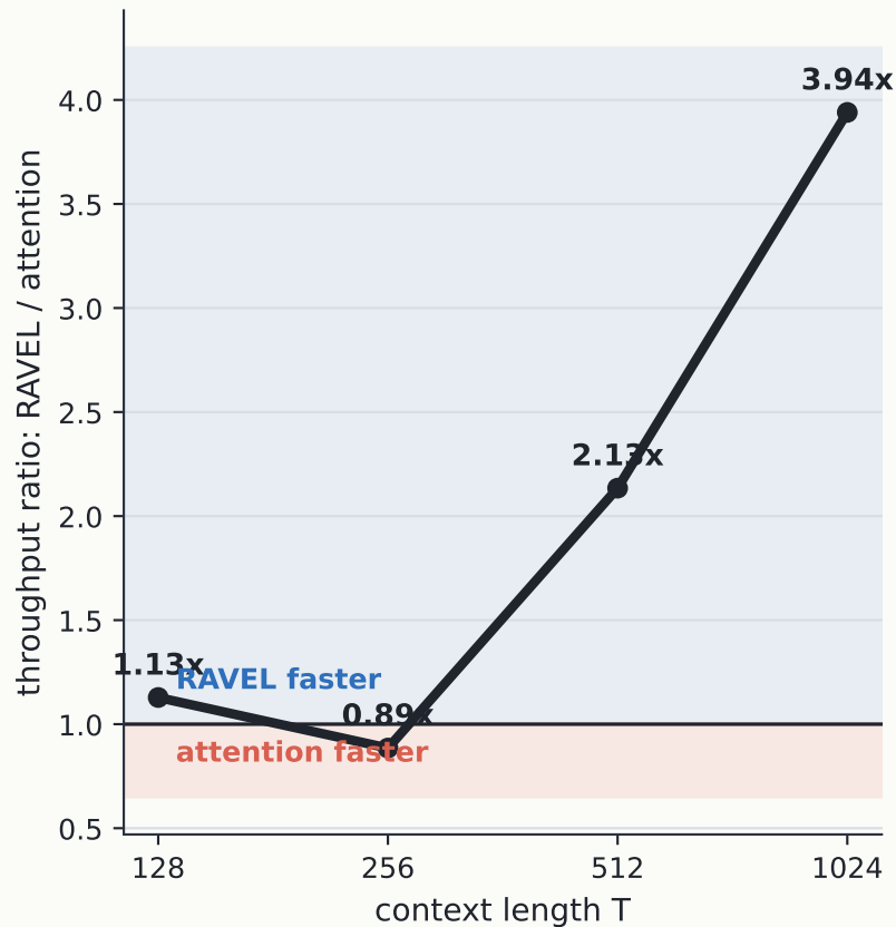
Crossover follows context length
