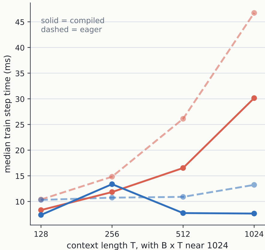
Attention step time bends upward with context
