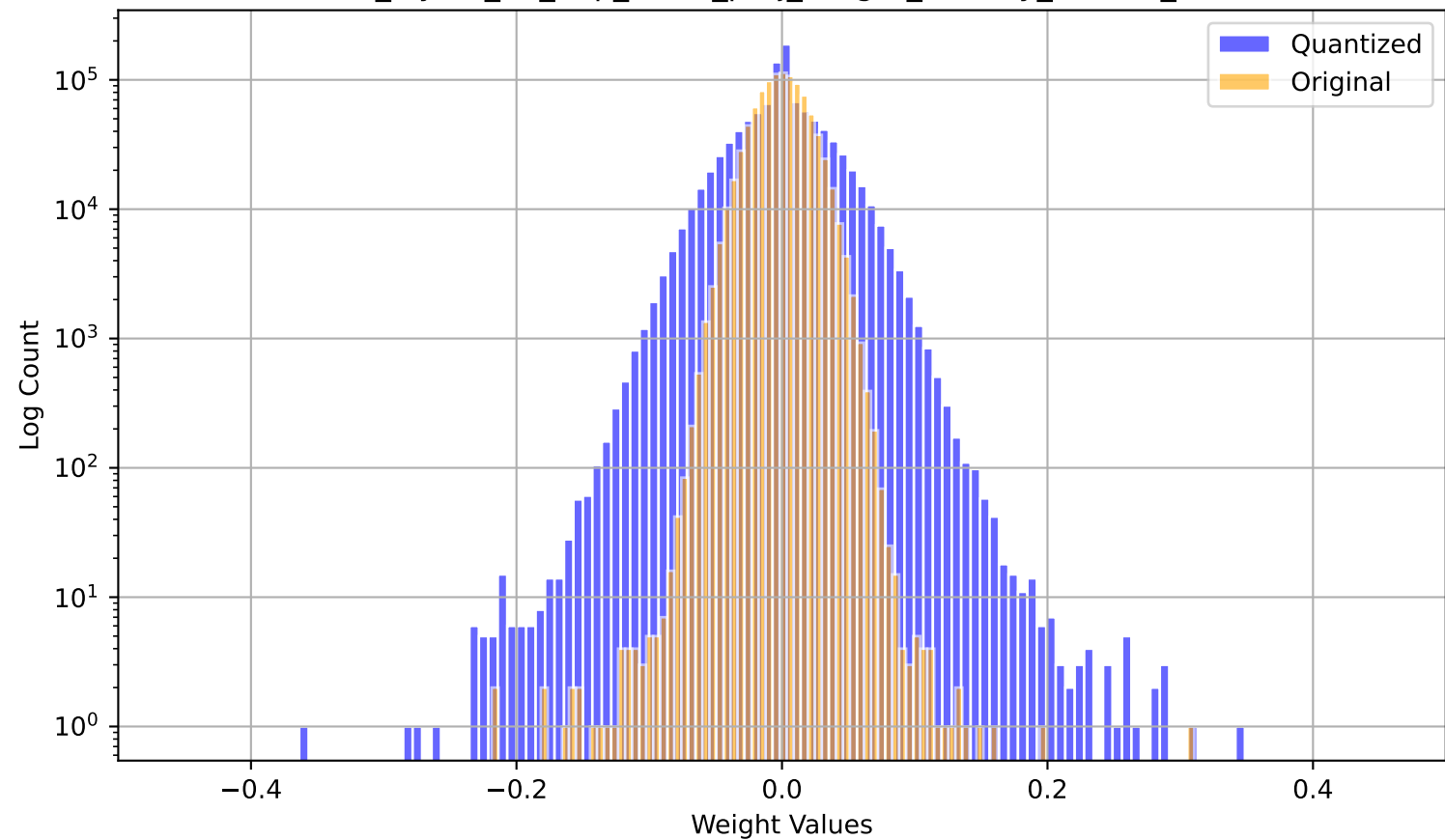
model_layers_30_mlp_down_proj_weight_overlay_3.0766_2.1431
