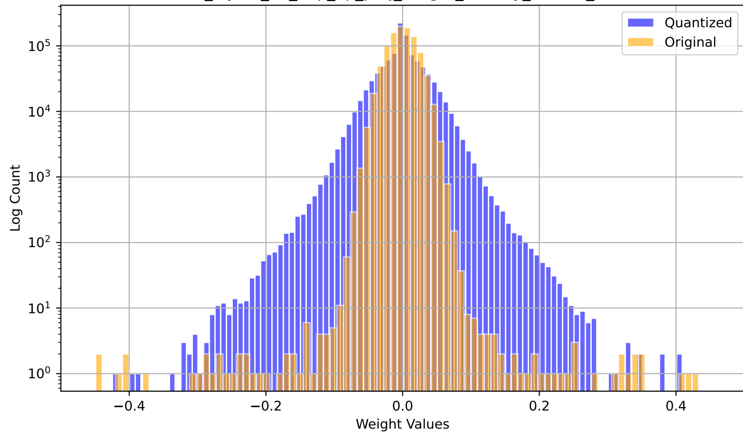
model_layers_30_mlp_up_proj_weight_overlay_3.4604_2.6230
