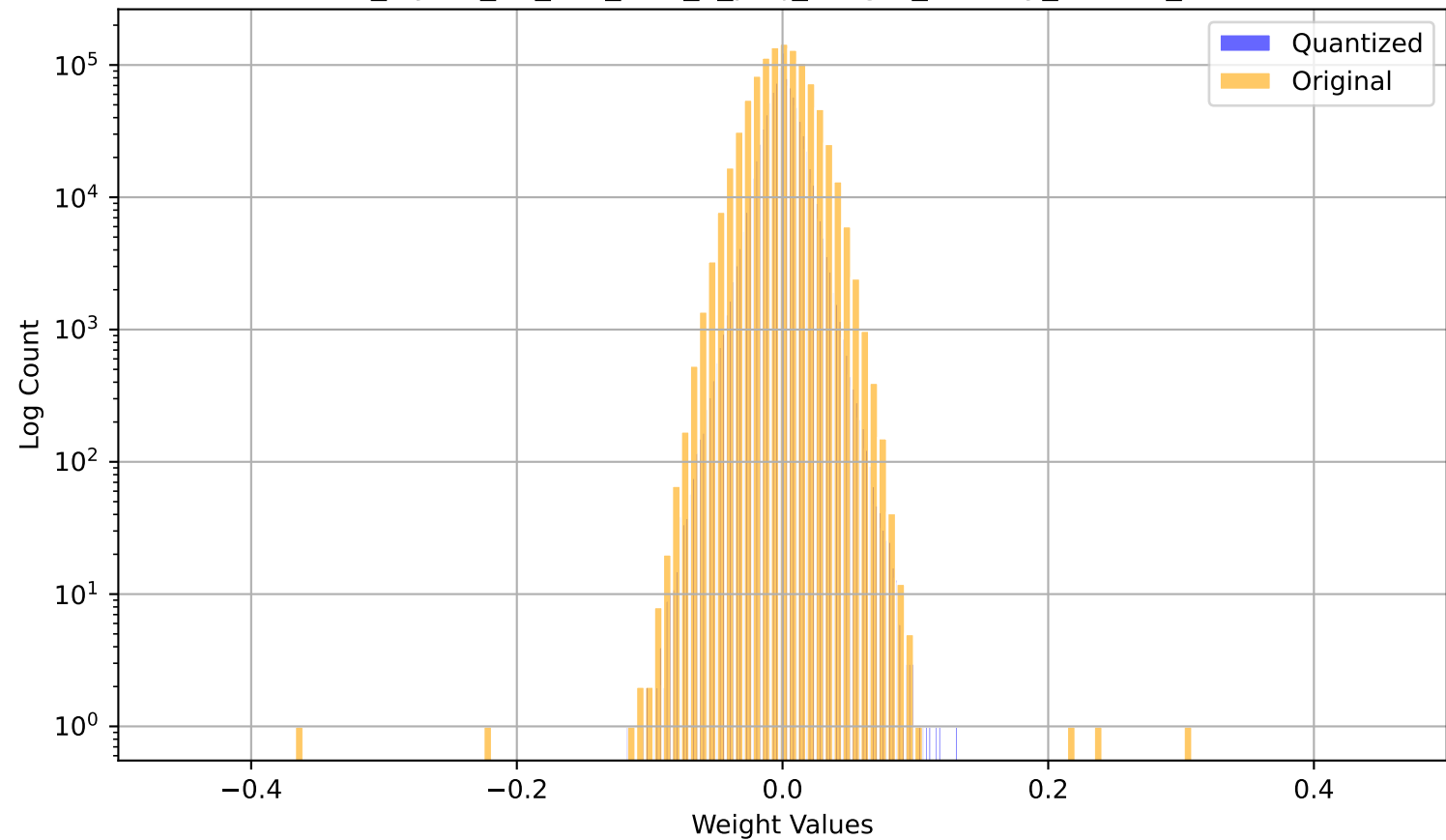
model_layers_31_self_attn_v_proj_weight_overlay_3.8706_3.2615
