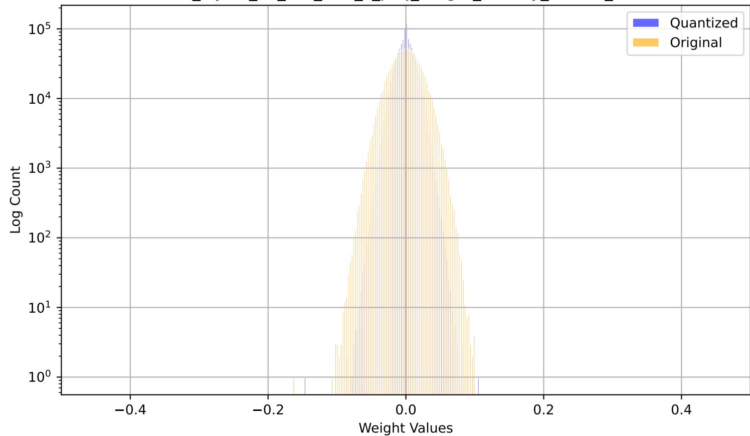
model_layers_30_self_attn_v_proj_weight_overlay_3.8398_3.1676
