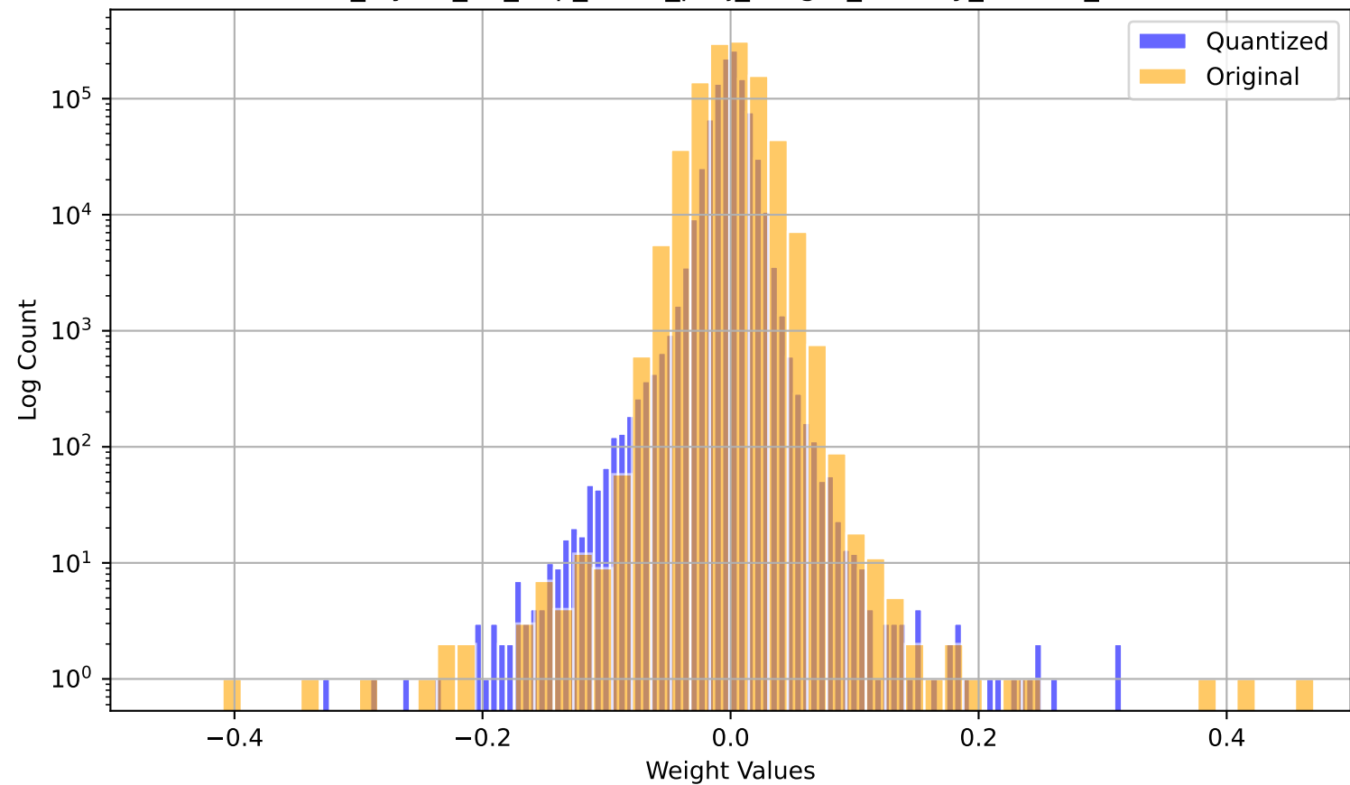
model_layers_31_mlp_down_proj_weight_overlay_2.4699_1.8470
