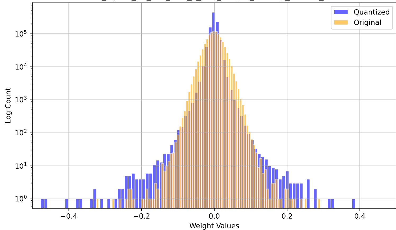
model_layers_31_self_attn_k_proj_weight_overlay_2.2650_3.3816
