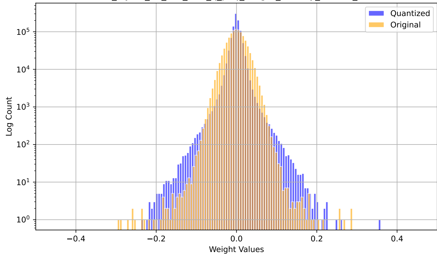
model_layers_31_self_attn_q_proj_weight_overlay_2.7198_3.0490
