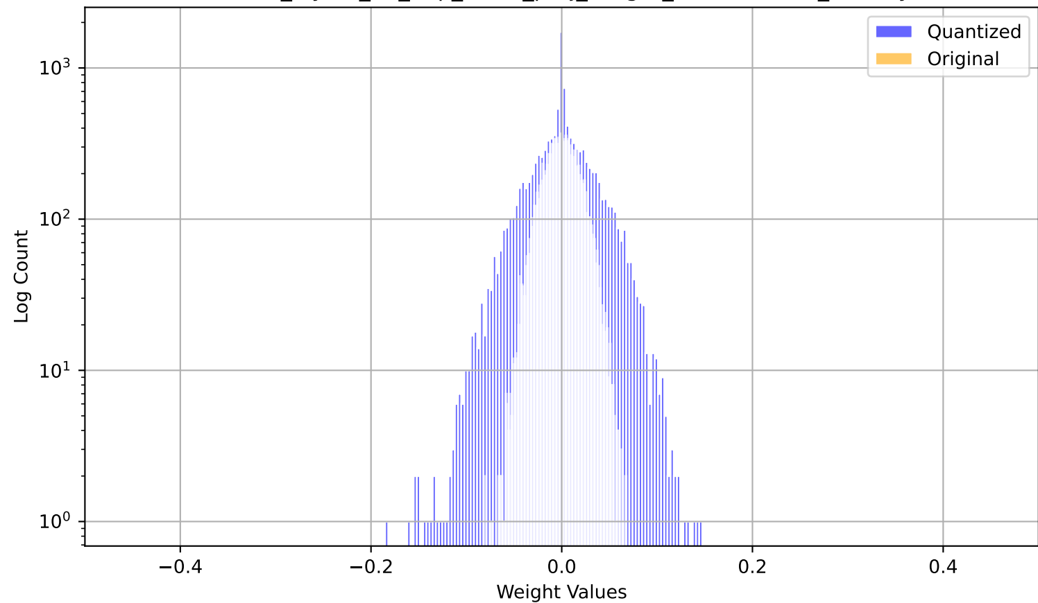
model_layers_30_mlp_down_proj_weight_channel1365_overlay
