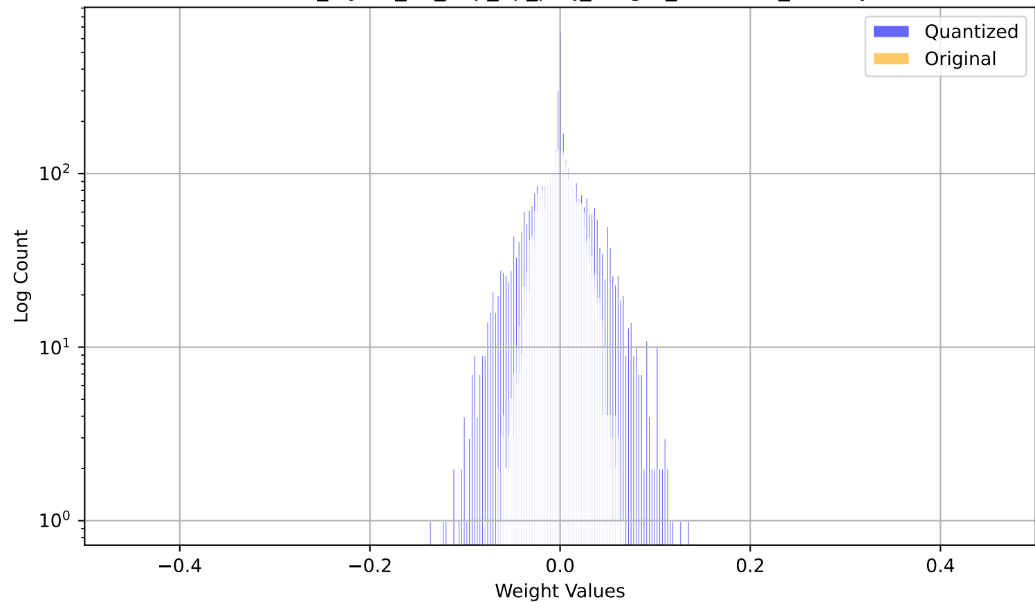
model_layers_30_mlp_up_proj_weight_channel0_overlay
