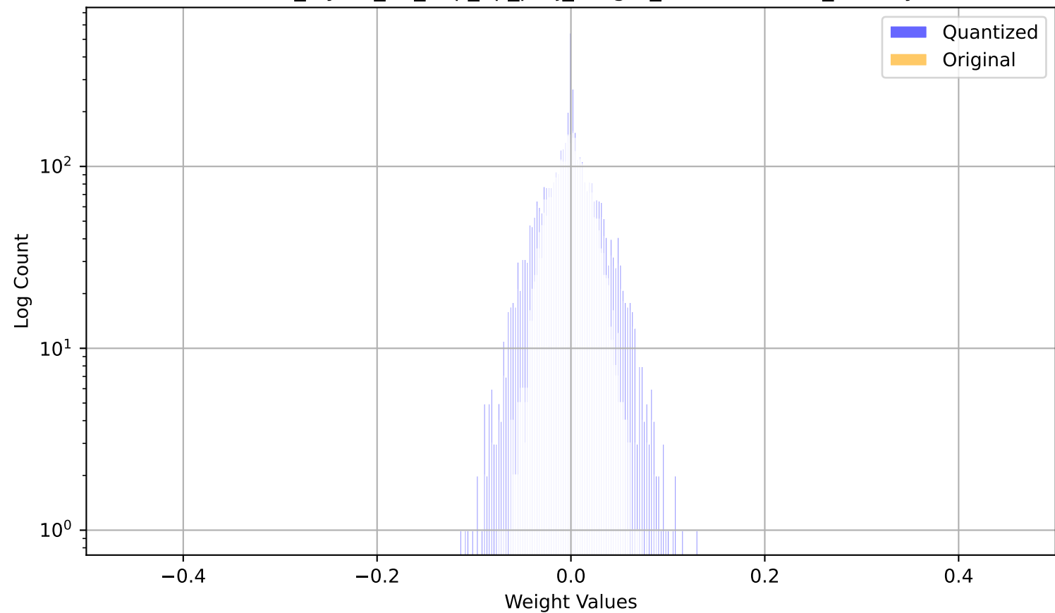
model_layers_30_mlp_up_proj_weight_channel11007_overlay
