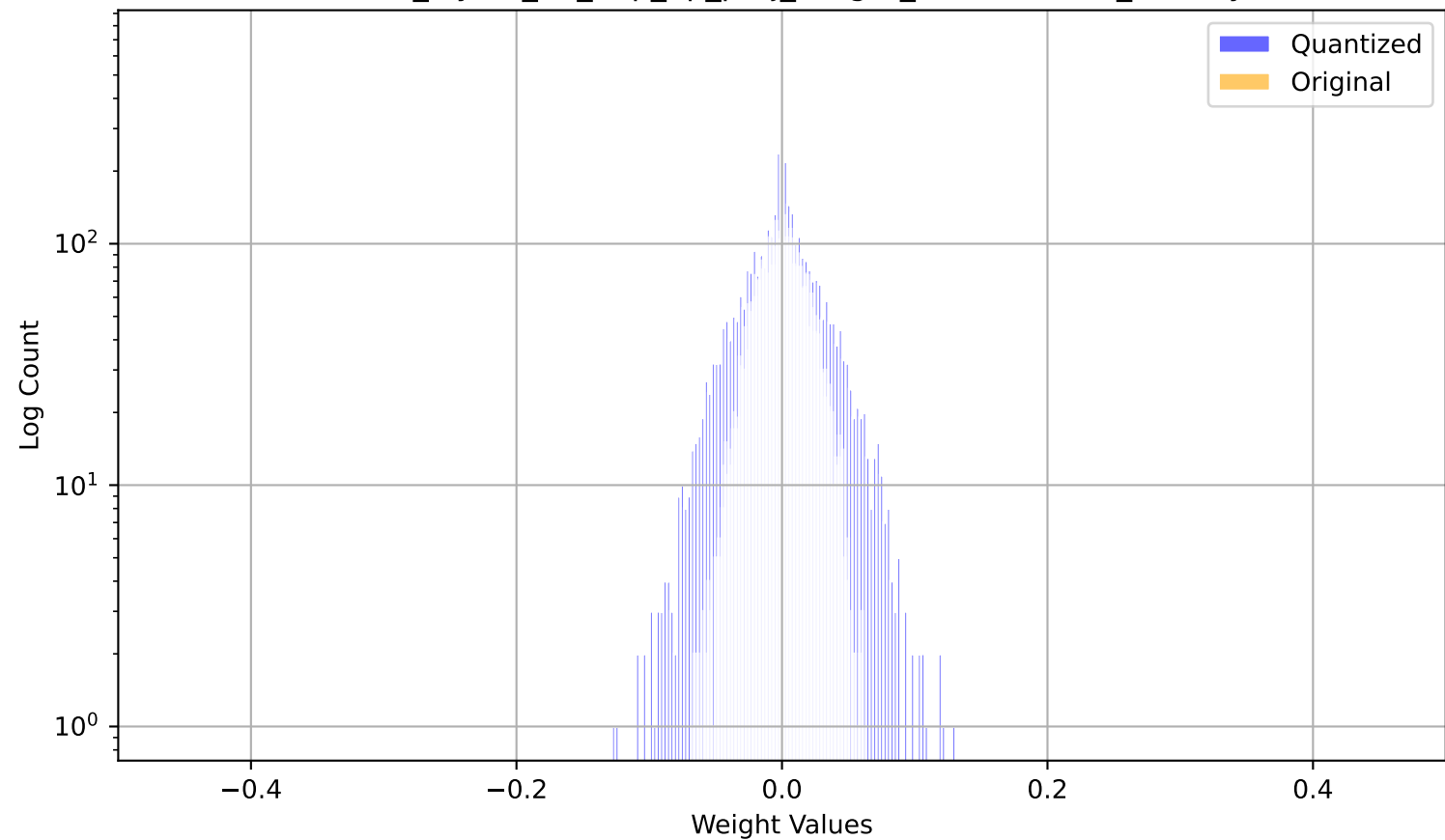
model_layers_30_mlp_up_proj_weight_channel2446_overlay
