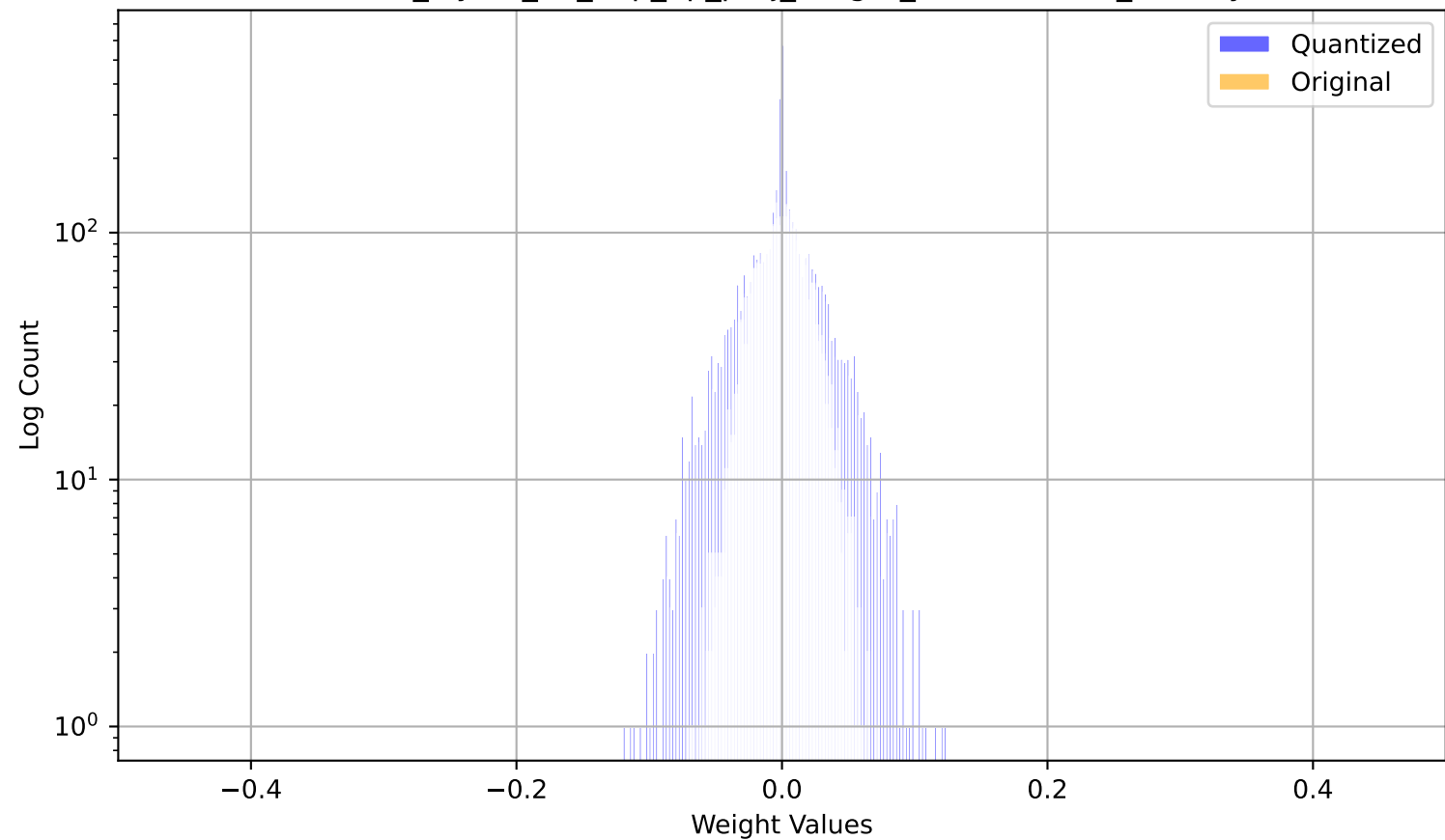
model_layers_30_mlp_up_proj_weight_channel4892_overlay
