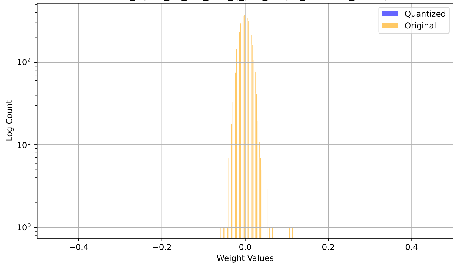
model_layers_31_self_attn_q_proj_weight_channel0_overlay
