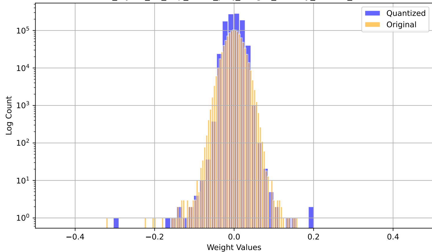
model_layers_30_mlp_down_proj_weight_overlay_2.0528_2.1431
