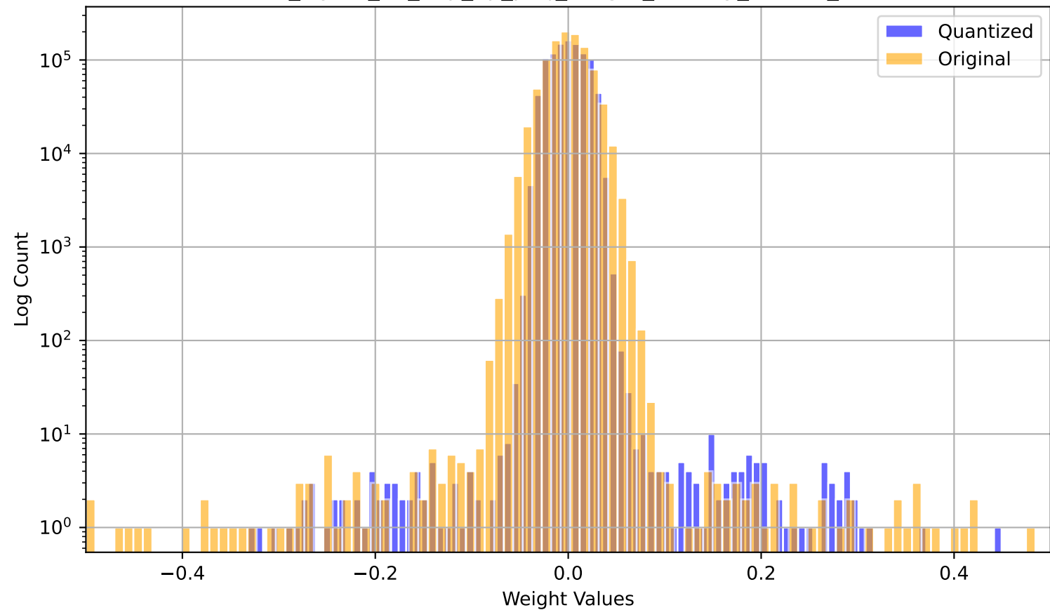
model_layers_30_mlp_up_proj_weight_overlay_2.5661_2.6230
