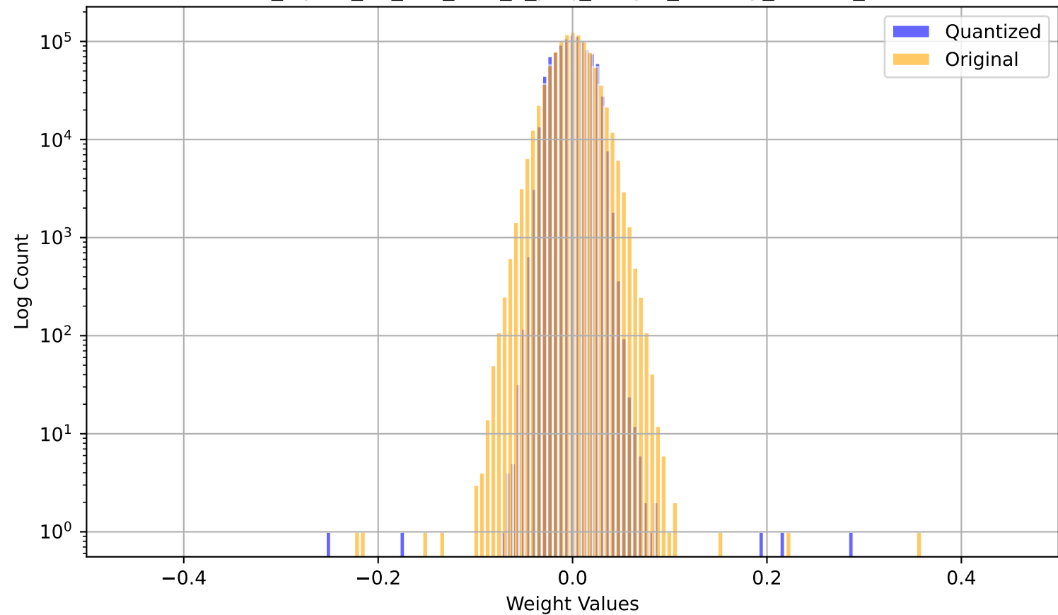
model_layers_31_self_attn_v_proj_weight_overlay_3.2204_3.2615
