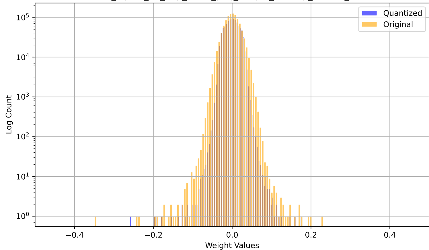
model_layers_31_mlp_down_proj_weight_overlay_1.8314_1.8470
