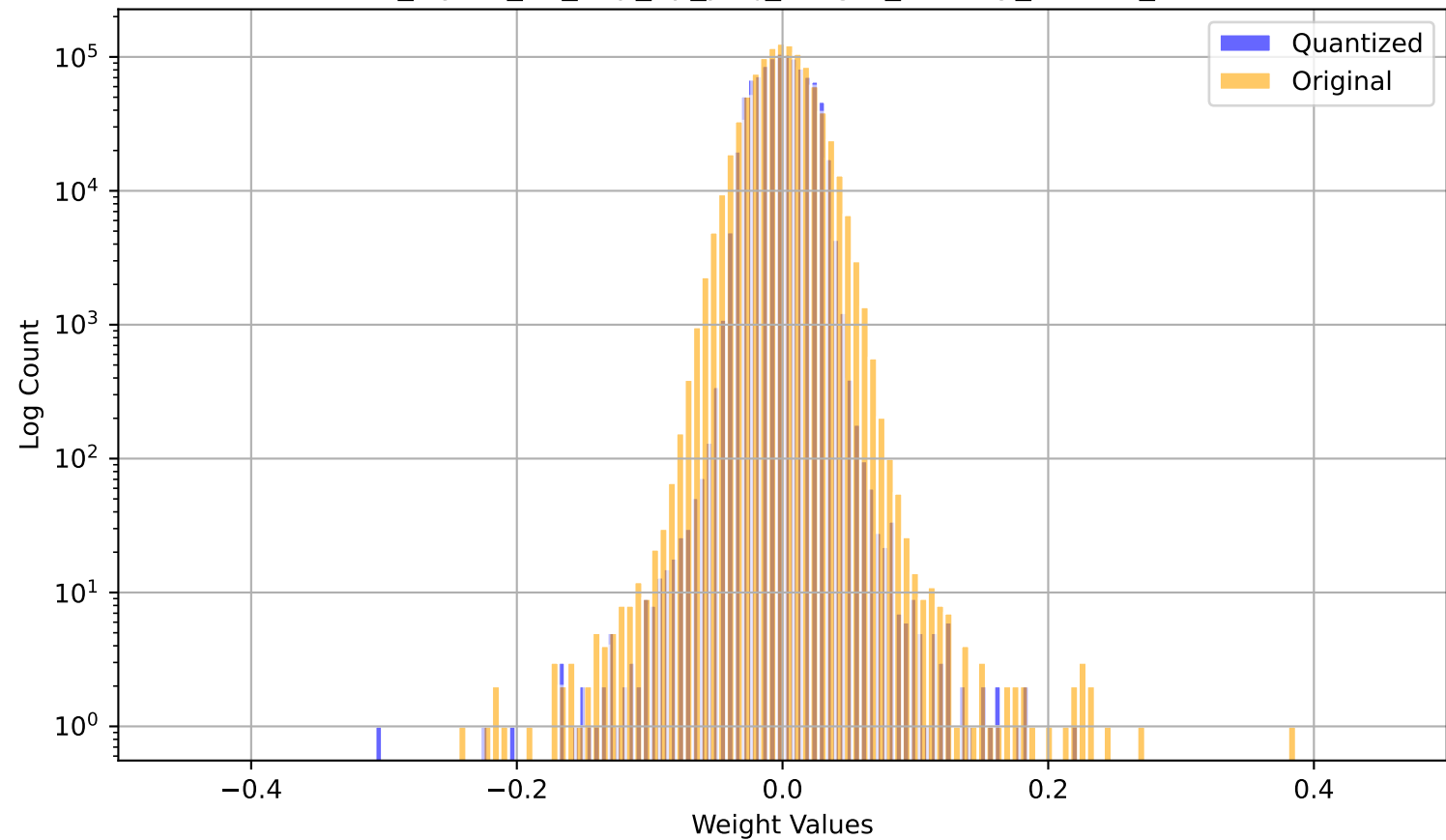
model_layers_31_mlp_up_proj_weight_overlay_2.6488_2.7779
