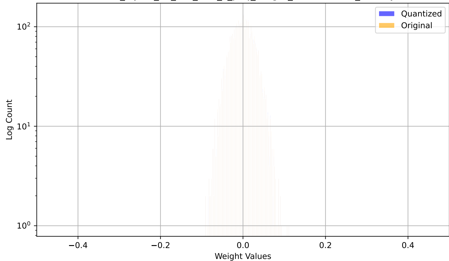
model_layers_31_self_attn_k_proj_weight_channel3640_overlay
