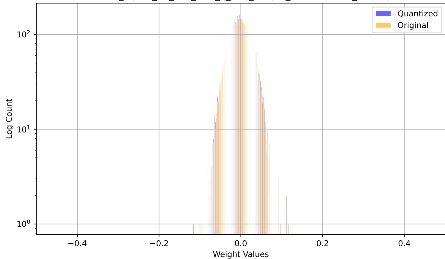
model_layers_31_self_attn_q_proj_weight_channel3640_overlay
