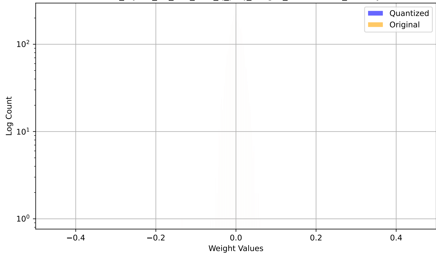
model_layers_31_self_attn_q_proj_weight_channel910_overlay
