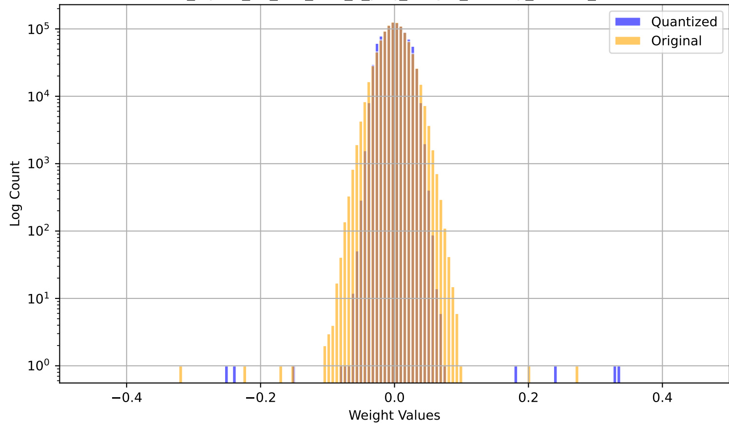
model_layers_31_self_attn_v_proj_weight_overlay_3.2555_3.2615
