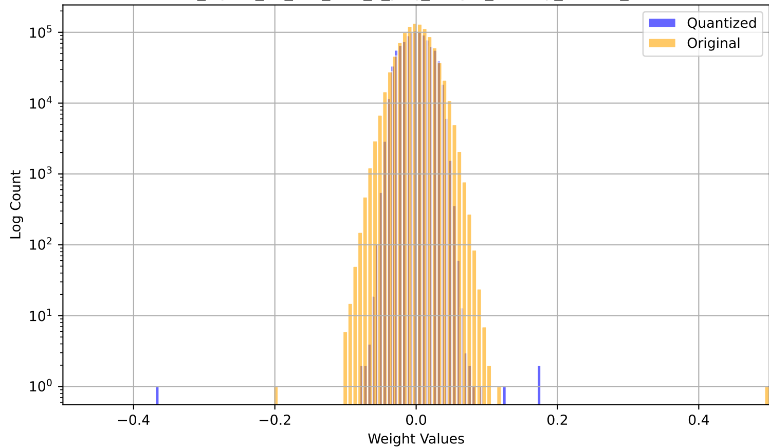
model_layers_30_self_attn_v_proj_weight_overlay_3.1449_3.1676
