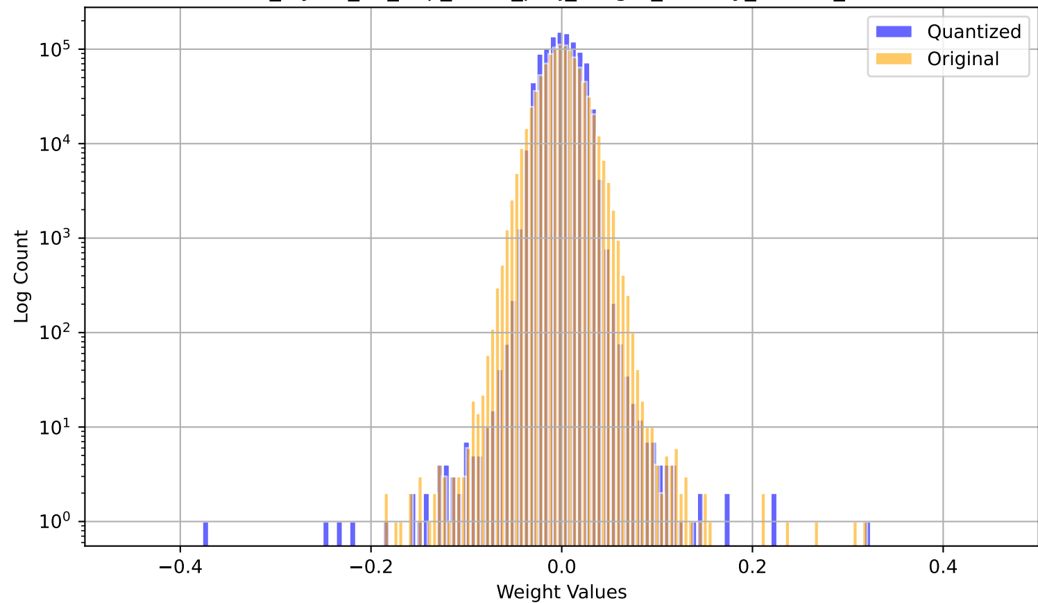
model_layers_31_mlp_down_proj_weight_overlay_1.8206_1.8470
