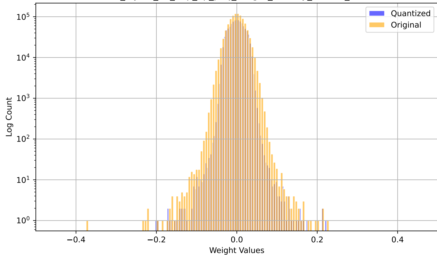
model_layers_31_mlp_up_proj_weight_overlay_2.8870_2.7779
