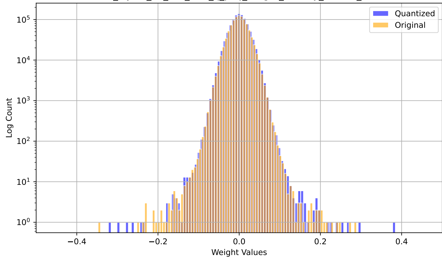
model_layers_31_self_attn_q_proj_weight_overlay_3.0490_3.0490
