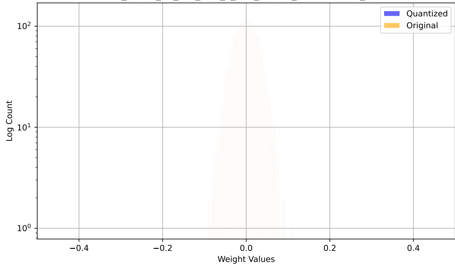
model_layers_31_self_attn_k_proj_weight_channel3640_overlay
